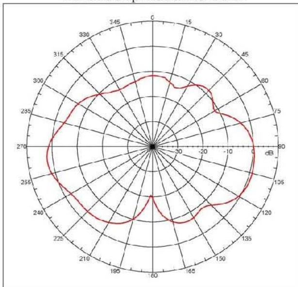
Far-field amplitude of AG-08.nsi
